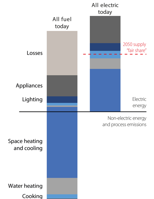
Figure 2.2: Energy use in buildings
