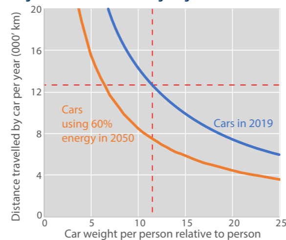
Figure 2.6: Car travel - trading weight and distance
